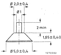
detail of side contact
