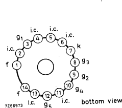
Fig. 5 Pin arrangement; bottom view.
