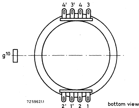
Fig. 10 Bottom view.
