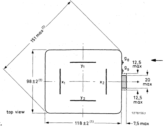
Fig. 3 Top view.
