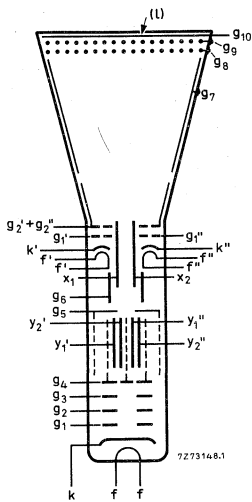
Fig. 4 Electrode configuration.
