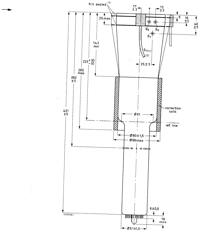
Fig. 1 Outlines.
