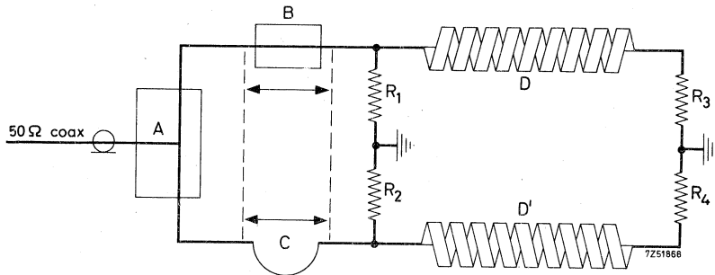
Fig.2 Connection to an asymmetrical 50 \Omega input
