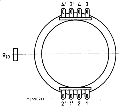
Fig. 10 Bottom view.
