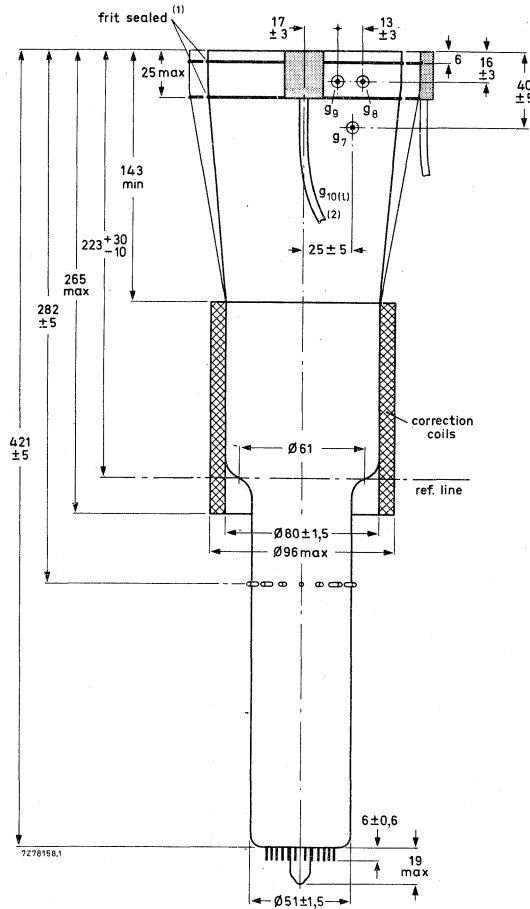
Fig. 1 Outlines.
